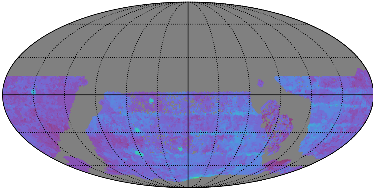
all_long_v3.4_10yrs WFD u band: 80thPercentile Season Length
