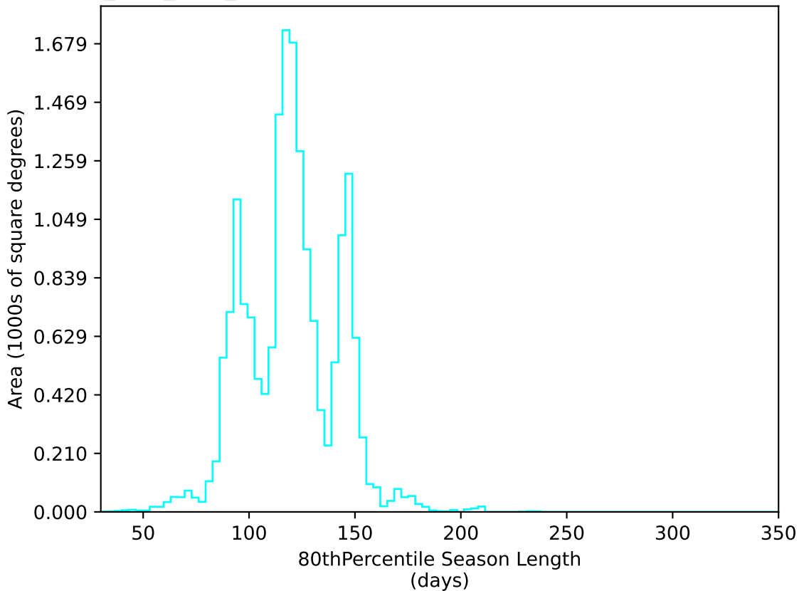
all_long_v3.4_10yrs WFD u band: 80thPercentile Season Length
