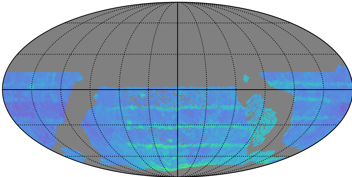
all_long_v3.4_10yrs WFD r band: 80thPercentile Season Length
