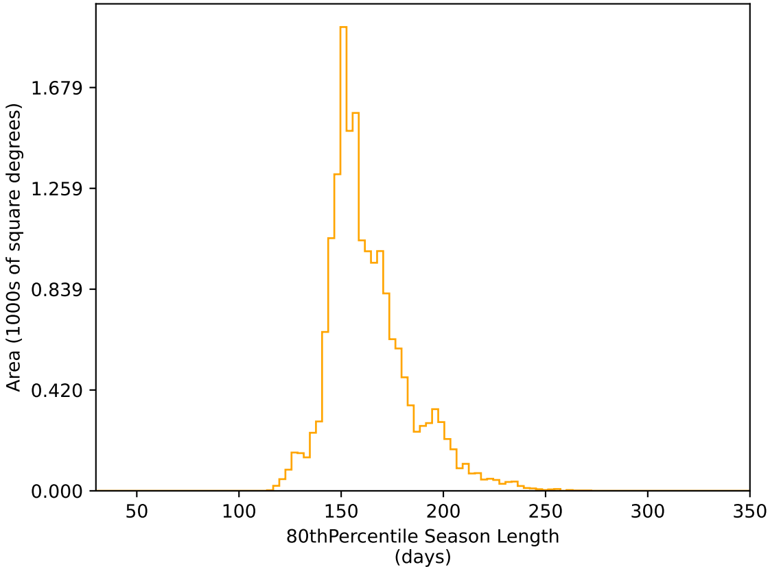
all_long_v3.4_10yrs WFD r band: 80thPercentile Season Length
