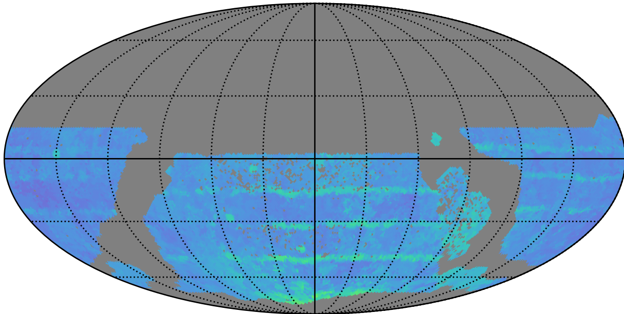
all_long_v3.4_10yrs WFD i band: 80thPercentile Season Length
