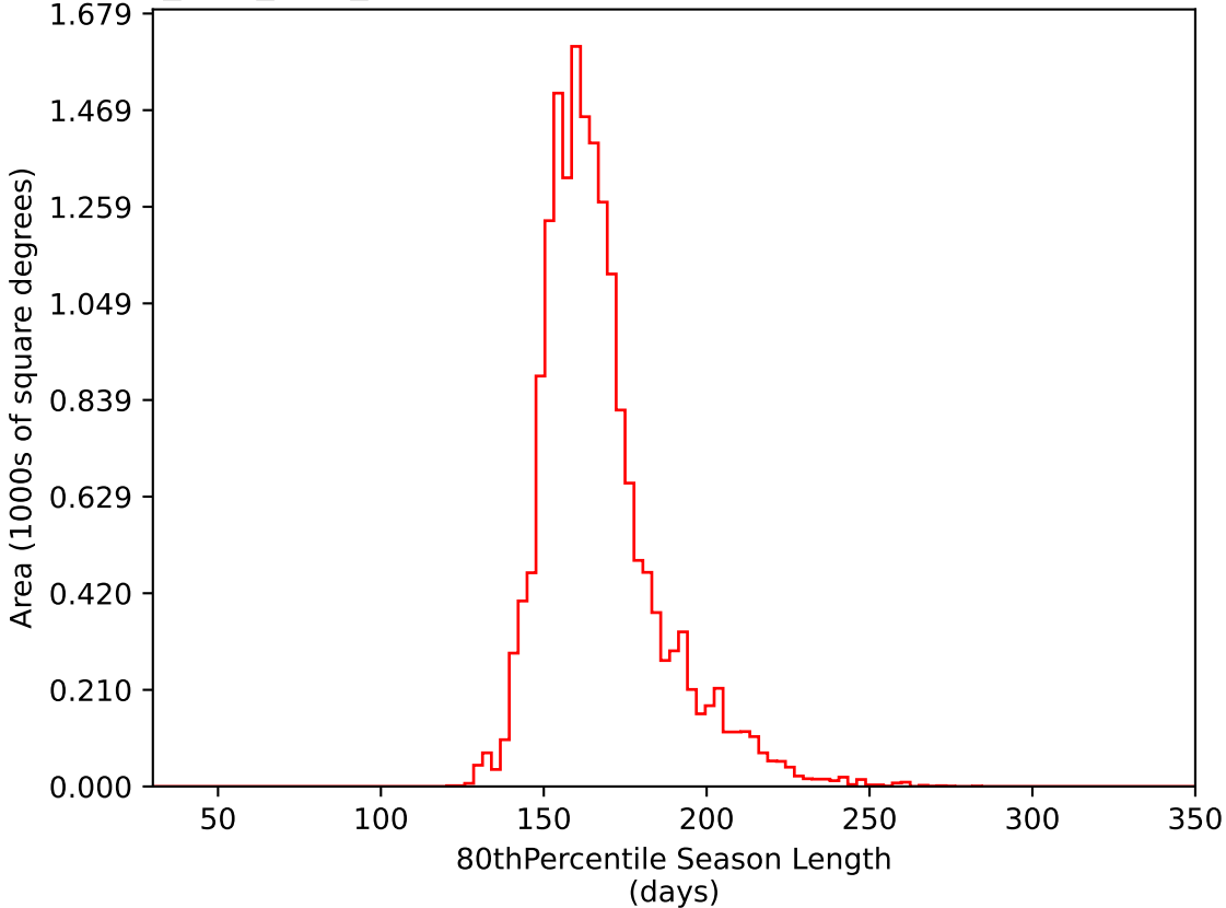
all_long_v3.4_10yrs WFD i band: 80thPercentile Season Length
