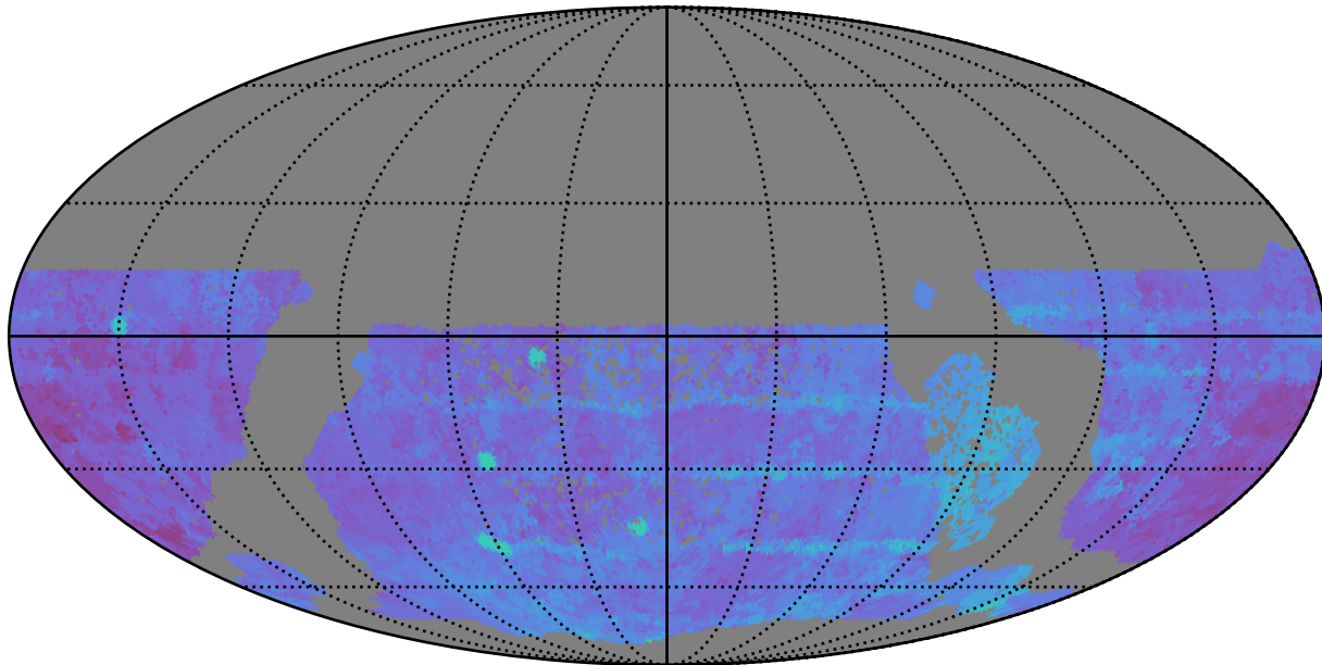
all_long_v3.4_10yrs WFD g band: 80thPercentile Season Length
