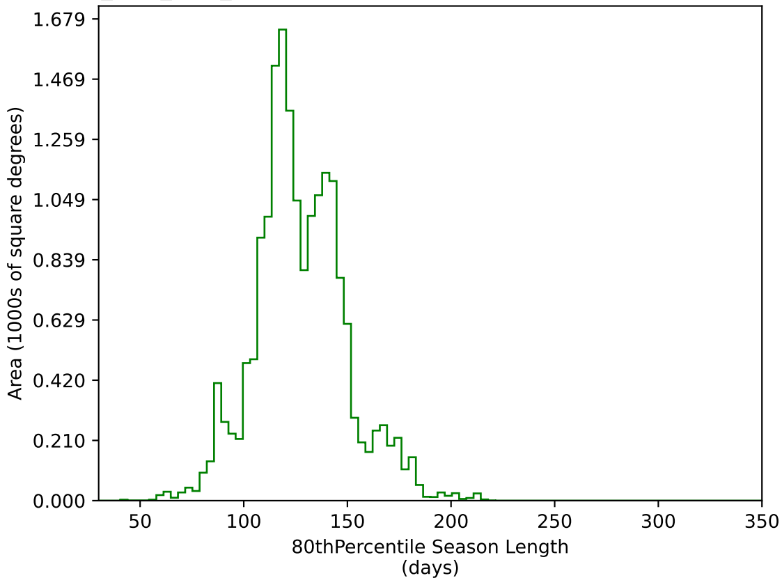
all_long_v3.4_10yrs WFD g band: 80thPercentile Season Length
