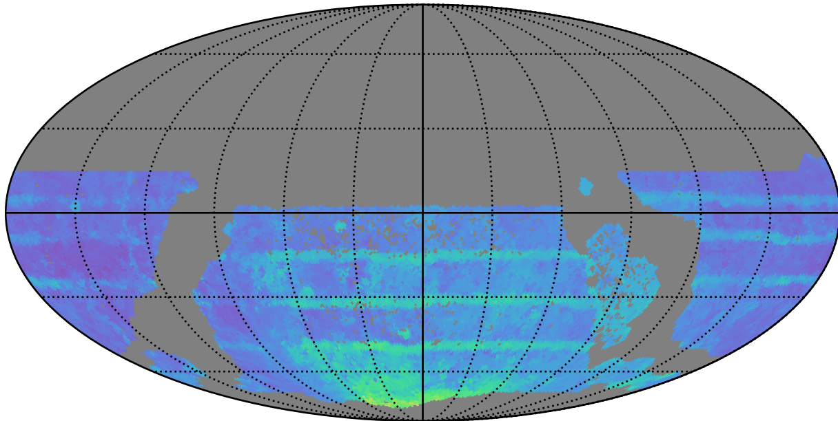
all_long_v3.4_10yrs WFD all bands: 80thPercentile Season Length
