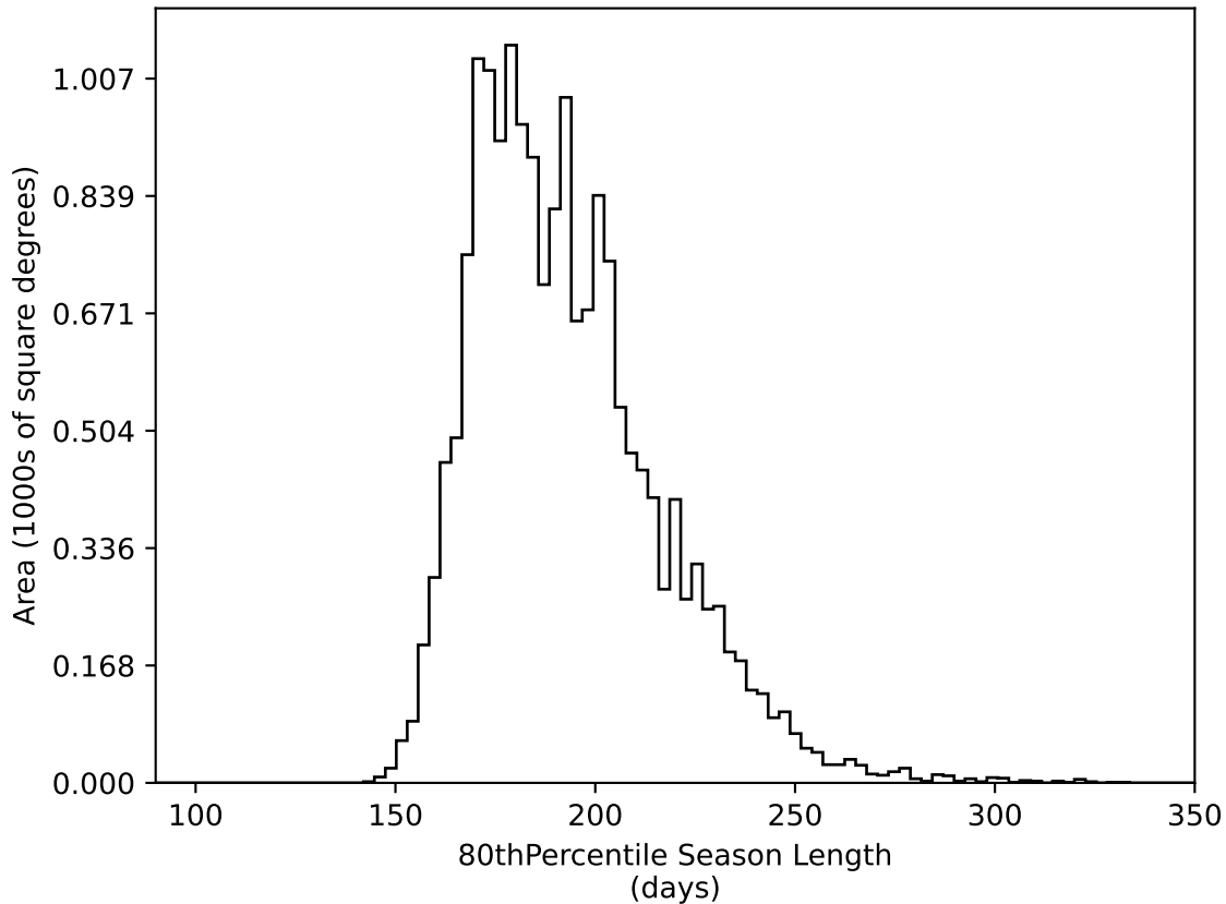
all_long_v3.4_10yrs WFD all bands: 80thPercentile Season Length
