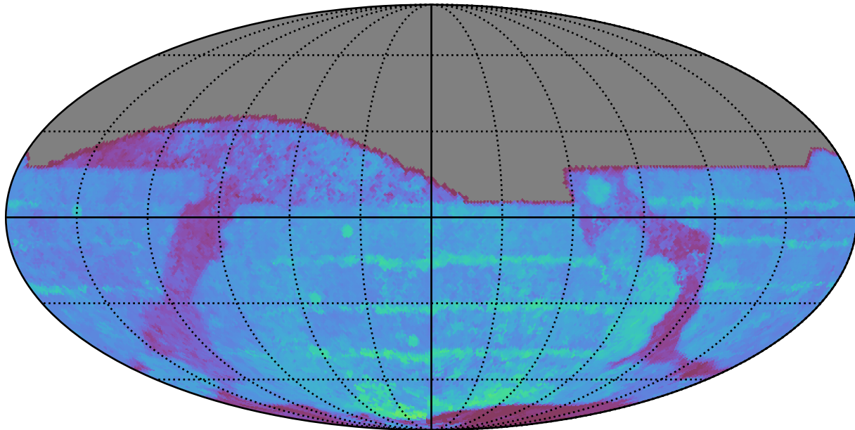
all_long_v3.4_10yrs All sky z band: 80thPercentile Season Length
