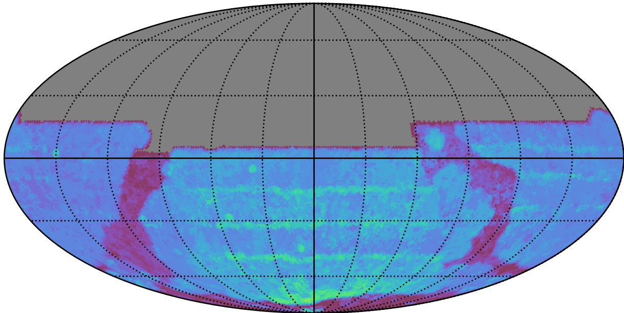
all_long_v3.4_10yrs All sky y band: 80thPercentile Season Length
