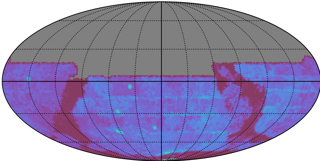
all_long_v3.4_10yrs All sky u band: 80thPercentile Season Length
