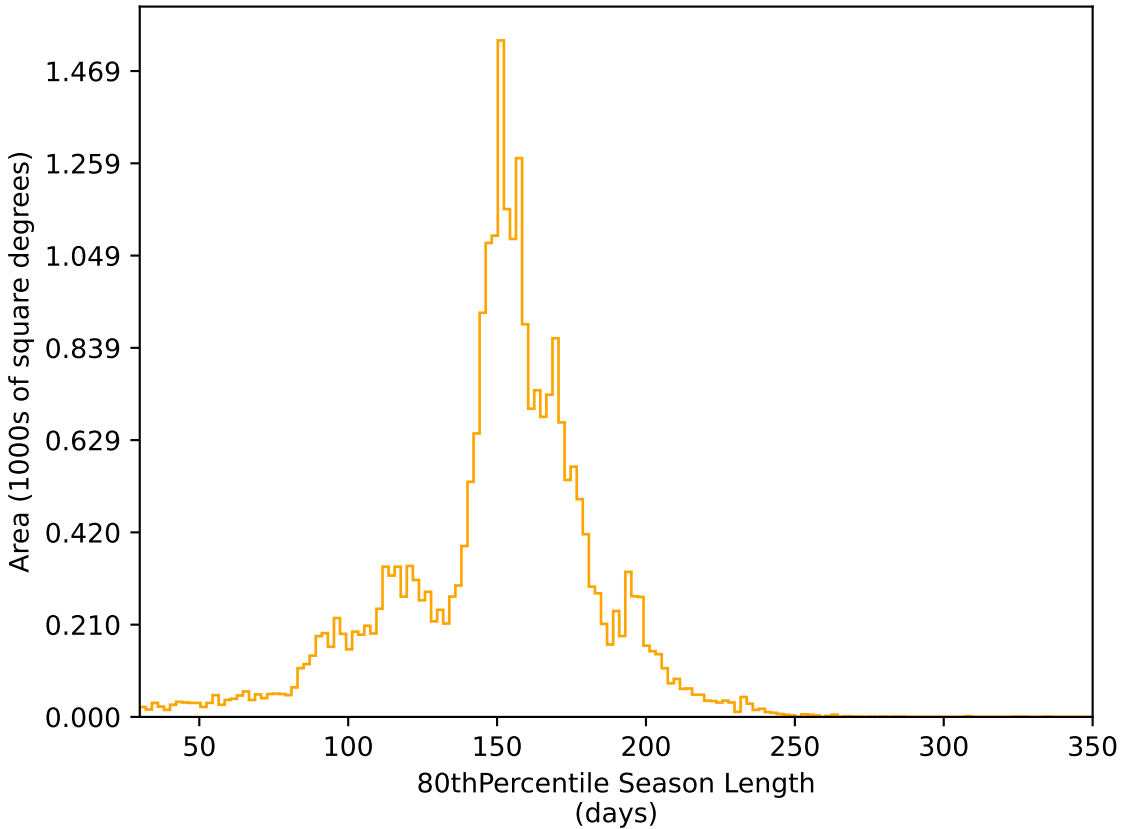
all_long_v3.4_10yrs All sky r band: 80thPercentile Season Length
