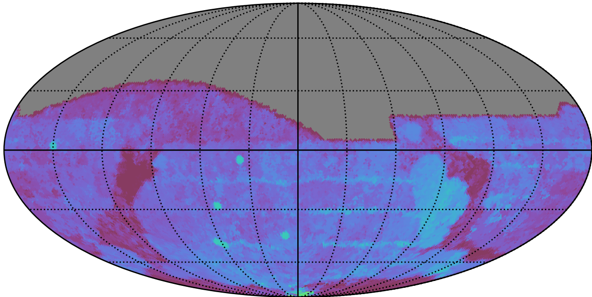
all_long_v3.4_10yrs All sky g band: 80thPercentile Season Length
