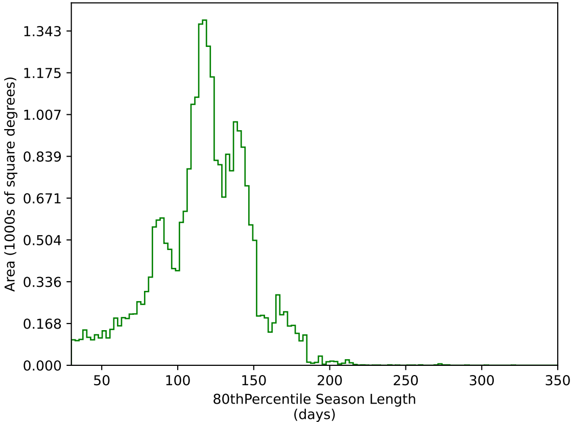
all_long_v3.4_10yrs All sky g band: 80thPercentile Season Length
