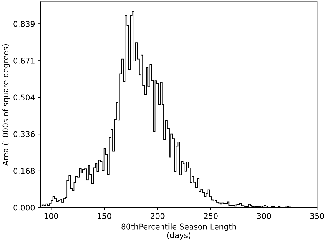
all_long_v3.4_10yrs All sky all bands: 80thPercentile Season Length
