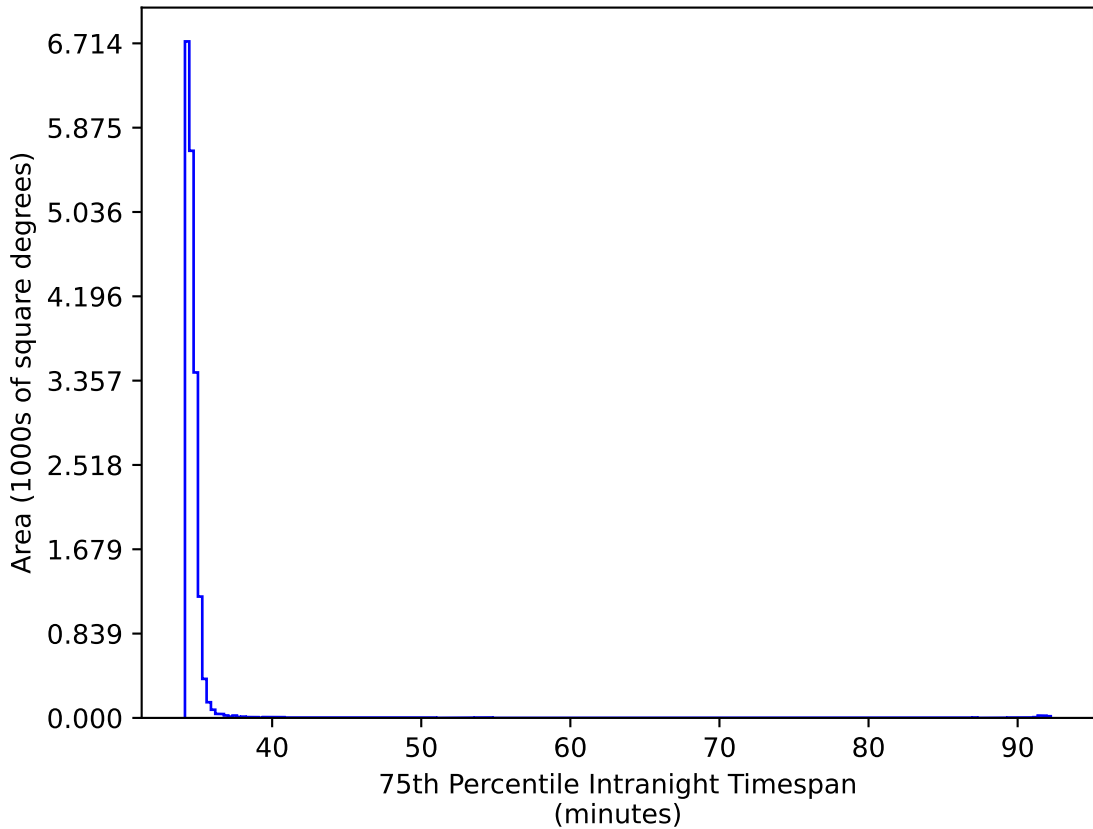
all_long_v3.4_10yrs WFD zy bands: 75th Percentile Intranight Timespan
