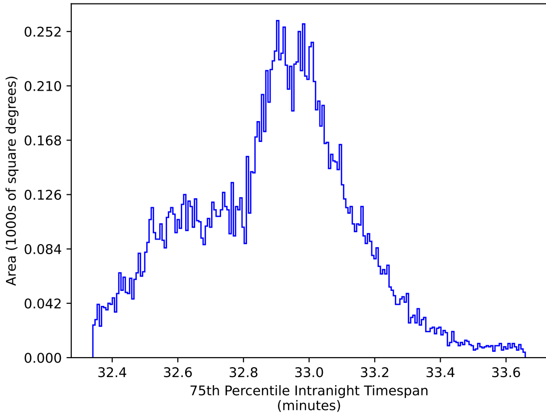
all_long_v3.4_10yrs WFD y band: 75th Percentile Intranight Timespan
