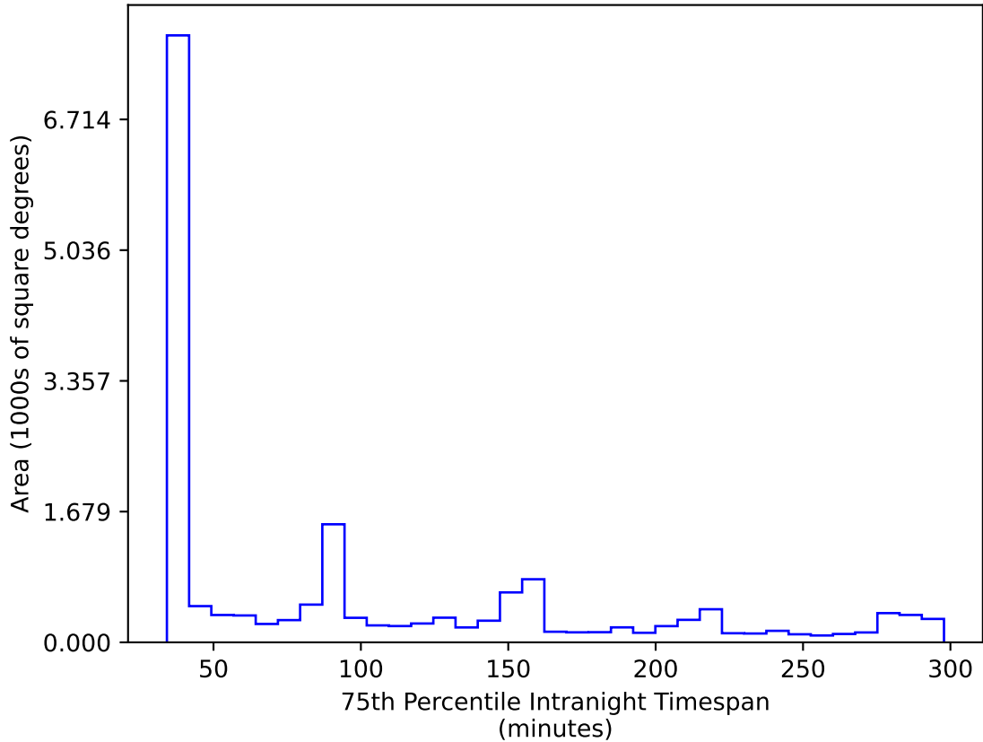
all_long_v3.4_10yrs WFD ri bands: 75th Percentile Intranight Timespan
