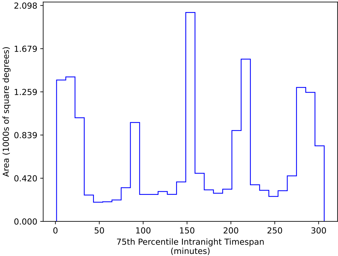
all_long_v3.4_10yrs WFD r band: 75th Percentile Intranight Timespan
