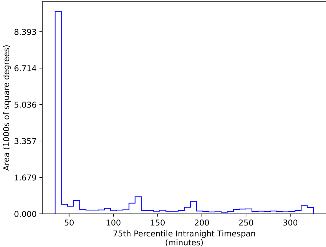
all_long_v3.4_10yrs WFD gr bands: 75th Percentile Intranight Timespan
