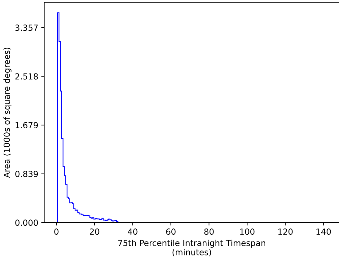
all_long_v3.4_10yrs WFD g band: 75th Percentile Intranight Timespan
