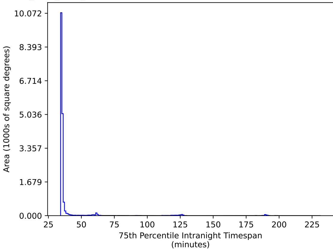
all_long_v3.4_10yrs WFD all bands: 75th Percentile Intranight Timespan
