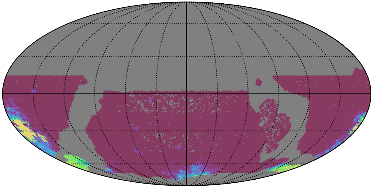
all_long_v3.4_10yrs WFD: 75th Percentile Intranight Timespan
