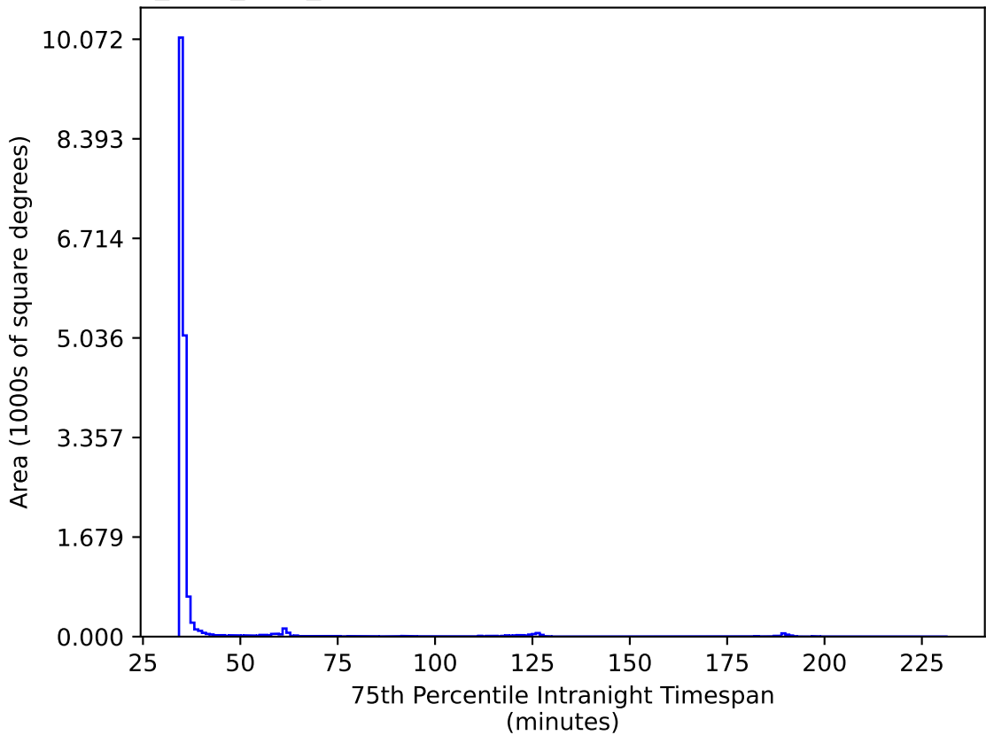
all_long_v3.4_10yrs WFD: 75th Percentile Intranight Timespan
