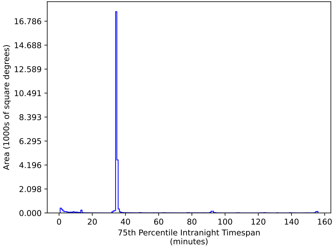
all_long_v3.4_10yrs All sky zy bands: 75th Percentile Intranight Timespan
