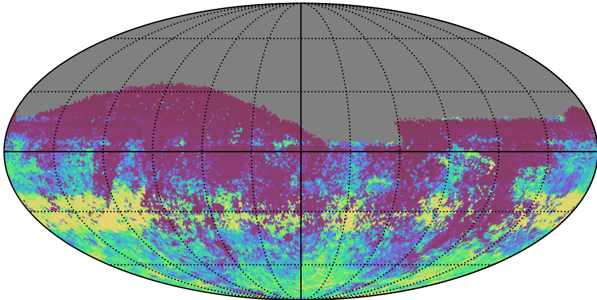
all_long_v3.4_10yrs All sky z band: 75th Percentile Intranight Timespan
