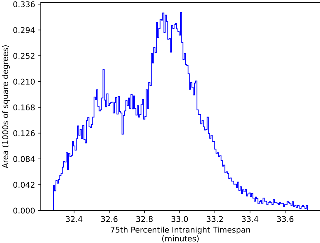
all_long_v3.4_10yrs All sky y band: 75th Percentile Intranight Timespan
