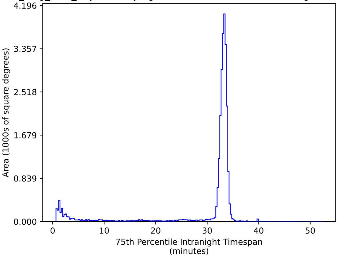
all_long_v3.4_10yrs All sky ug bands: 75th Percentile Intranight Timespan
