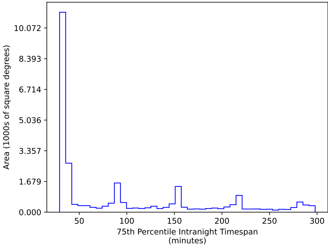
all_long_v3.4_10yrs All sky ri bands: 75th Percentile Intranight Timespan
