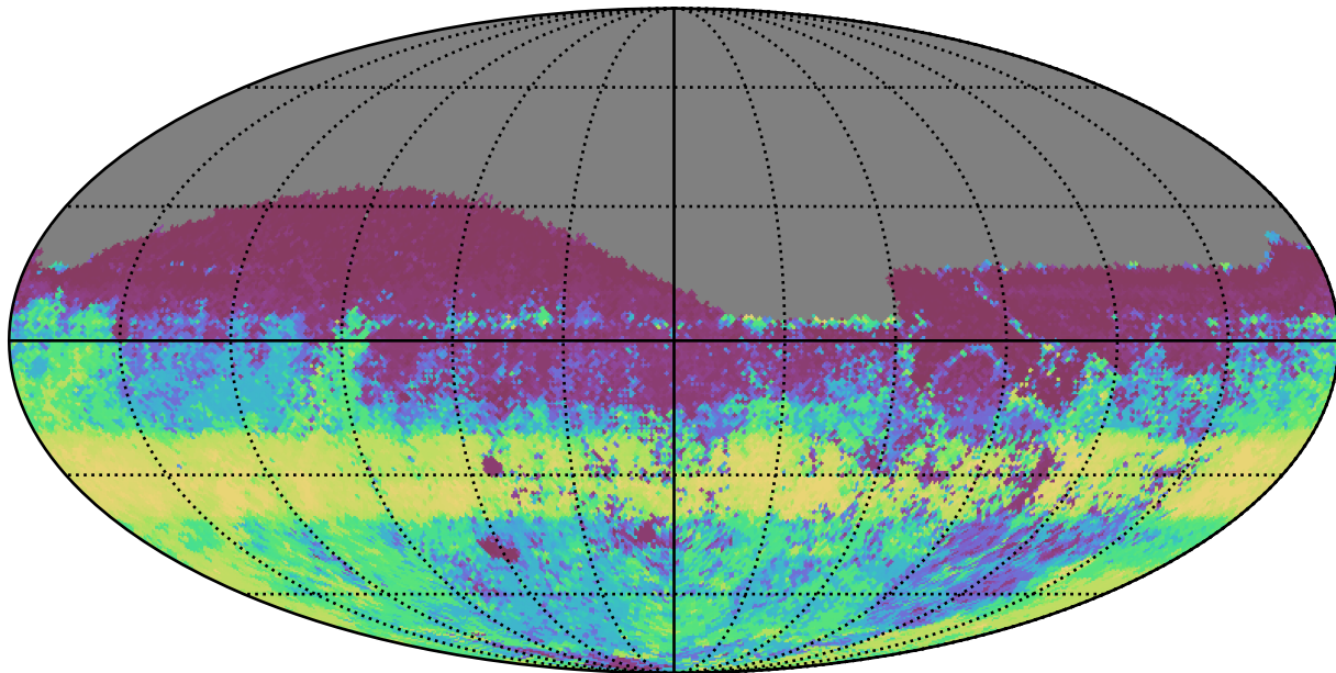
all_long_v3.4_10yrs All sky r band: 75th Percentile Intranight Timespan
