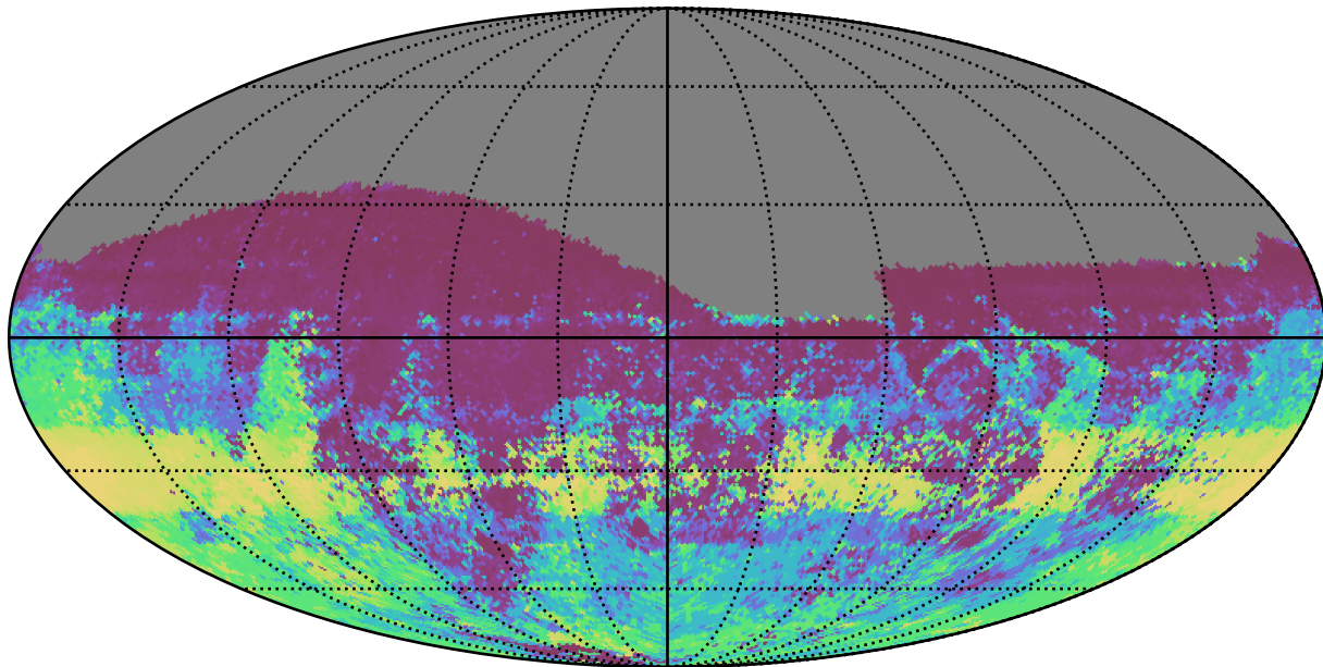
all_long_v3.4_10yrs All sky i band: 75th Percentile Intranight Timespan
