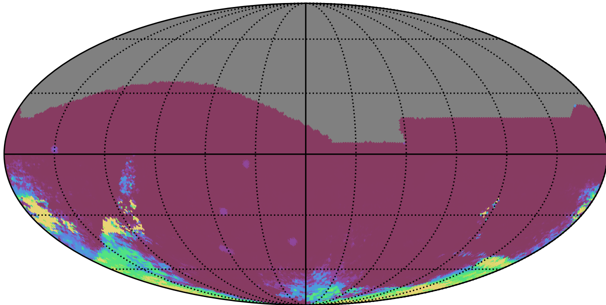
all_long_v3.4_10yrs All sky all bands: 75th Percentile Intranight Timespan
