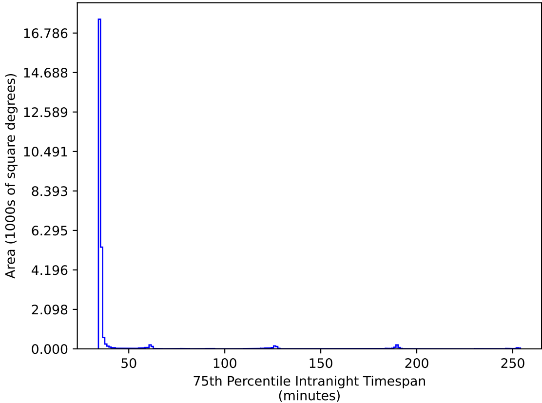
all_long_v3.4_10yrs All sky all bands: 75th Percentile Intranight Timespan
