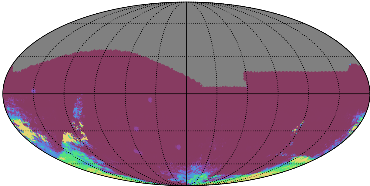
all_long_v3.4_10yrs All sky: 75th Percentile Intranight Timespan
