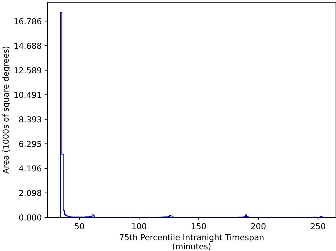
all_long_v3.4_10yrs All sky: 75th Percentile Intranight Timespan
