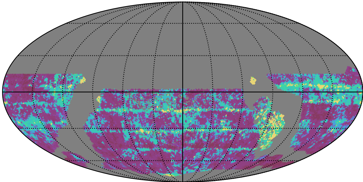
all_long_v3.4_10yrs WFD z band: 20thPercentile Inter-Night Gap
