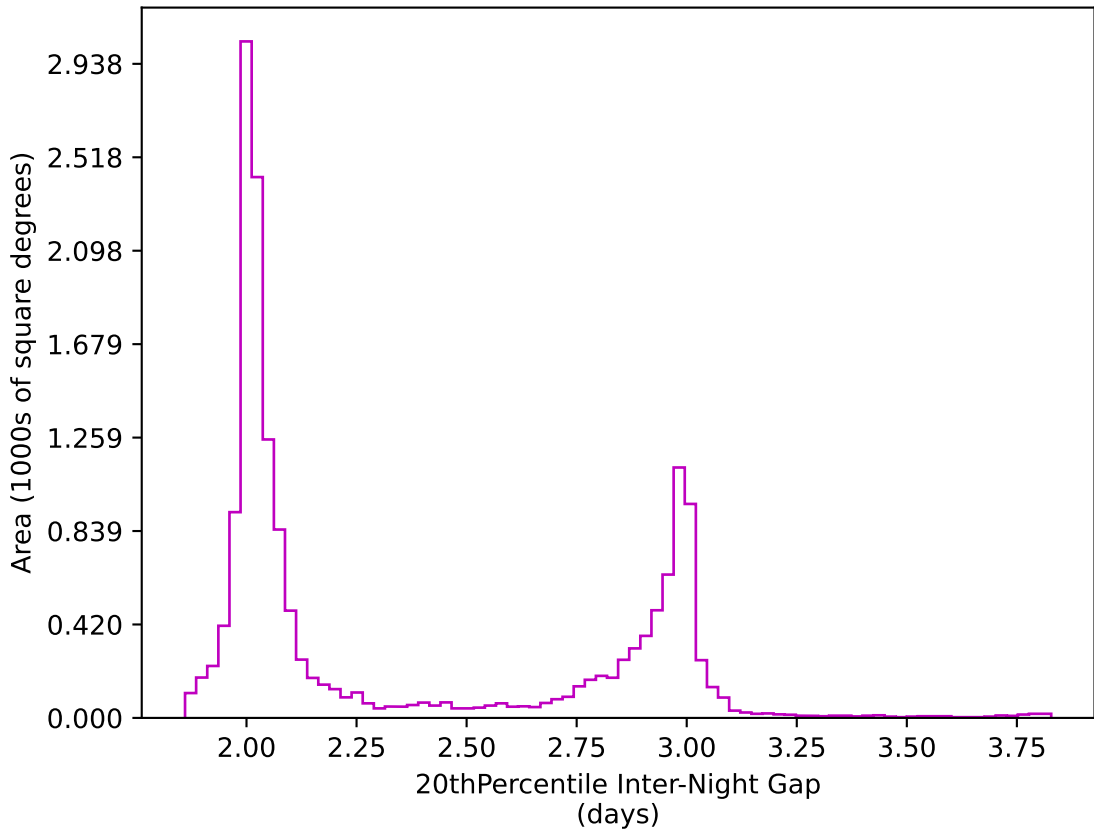
all_long_v3.4_10yrs WFD z band: 20thPercentile Inter-Night Gap
