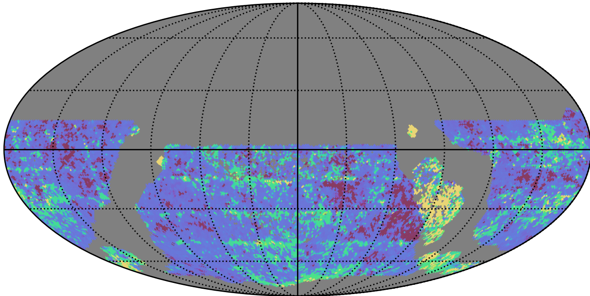
all_long_v3.4_10yrs WFD y band: 20thPercentile Inter-Night Gap
