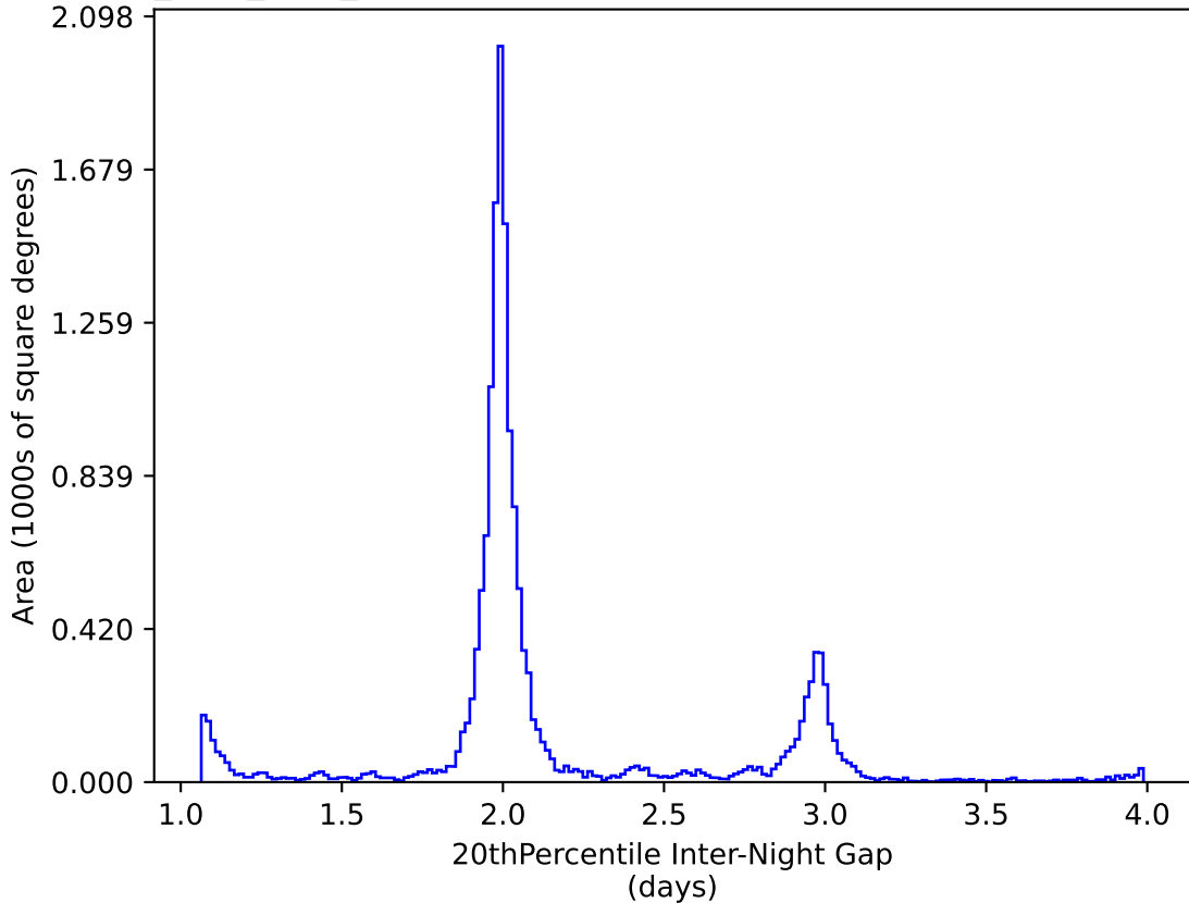
all_long_v3.4_10yrs WFD y band: 20thPercentile Inter-Night Gap
