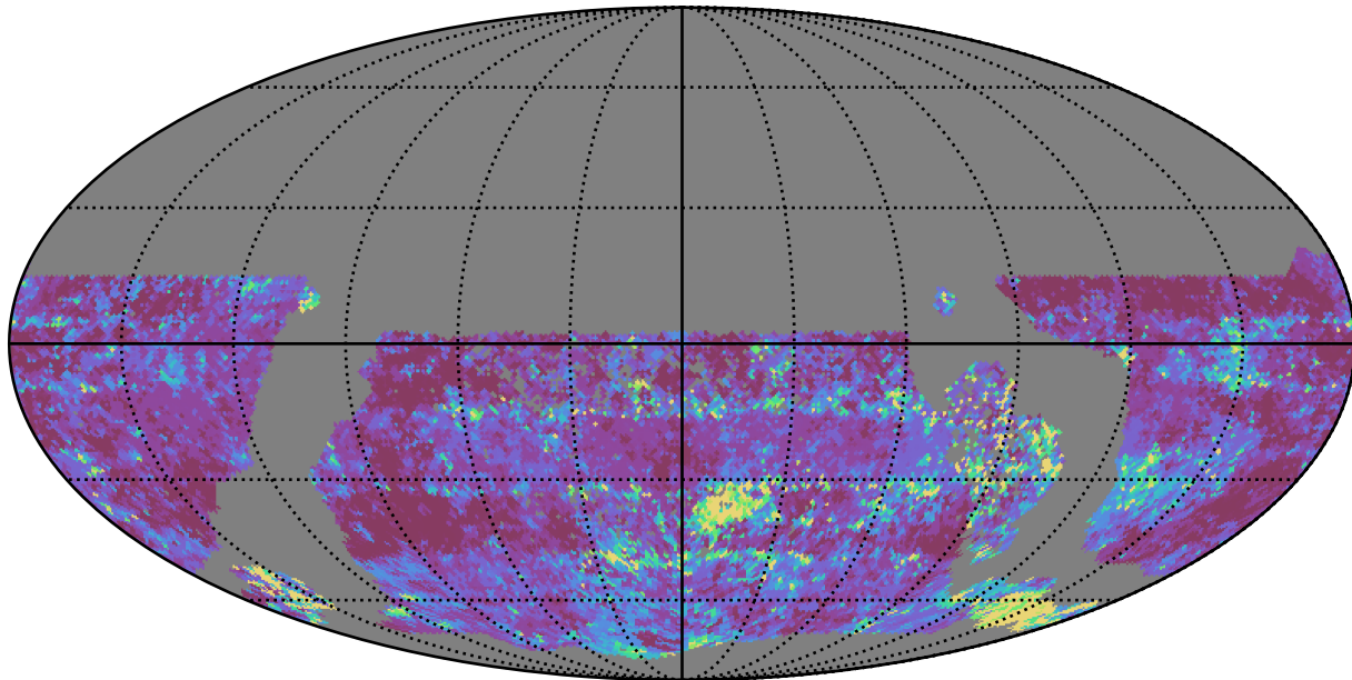
all_long_v3.4_10yrs WFD u band: 20thPercentile Inter-Night Gap
