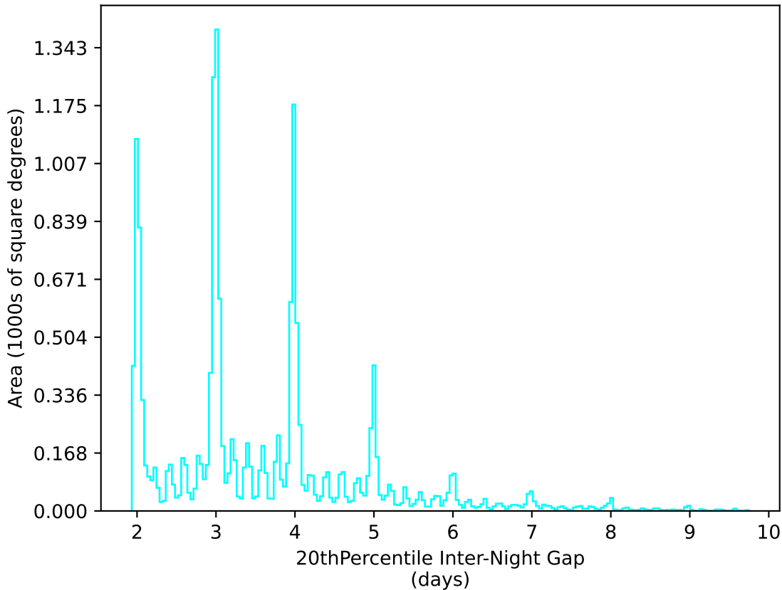
all_long_v3.4_10yrs WFD u band: 20thPercentile Inter-Night Gap
