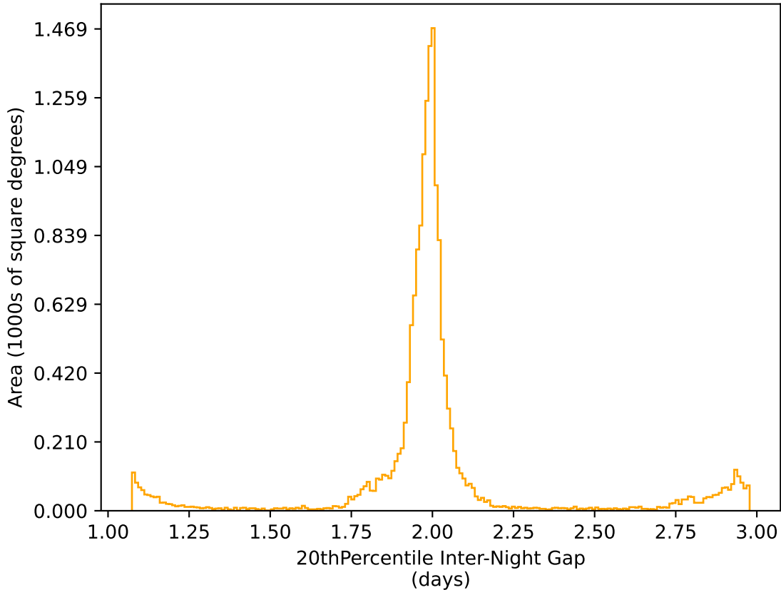
all_long_v3.4_10yrs WFD r band: 20thPercentile Inter-Night Gap
