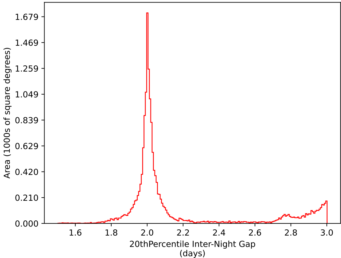
all_long_v3.4_10yrs WFD i band: 20thPercentile Inter-Night Gap
