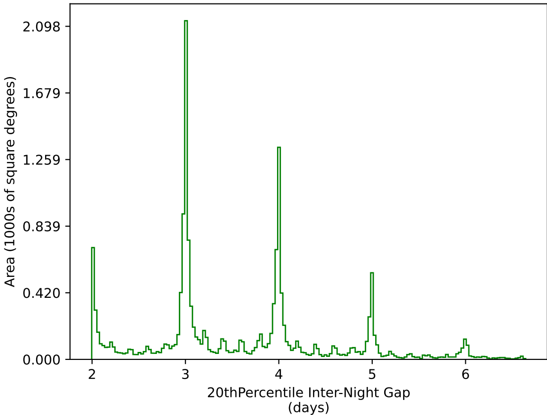
all_long_v3.4_10yrs WFD g band: 20thPercentile Inter-Night Gap
