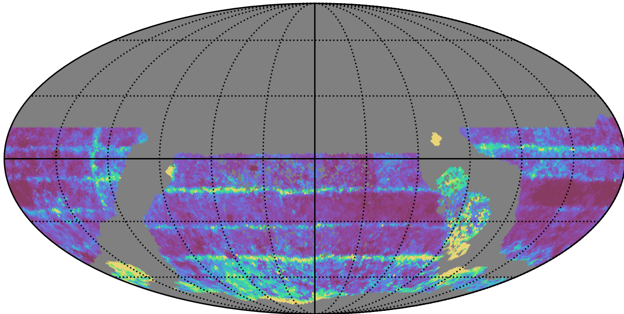
all_long_v3.4_10yrs WFD all bands: 20thPercentile Inter-Night Gap
