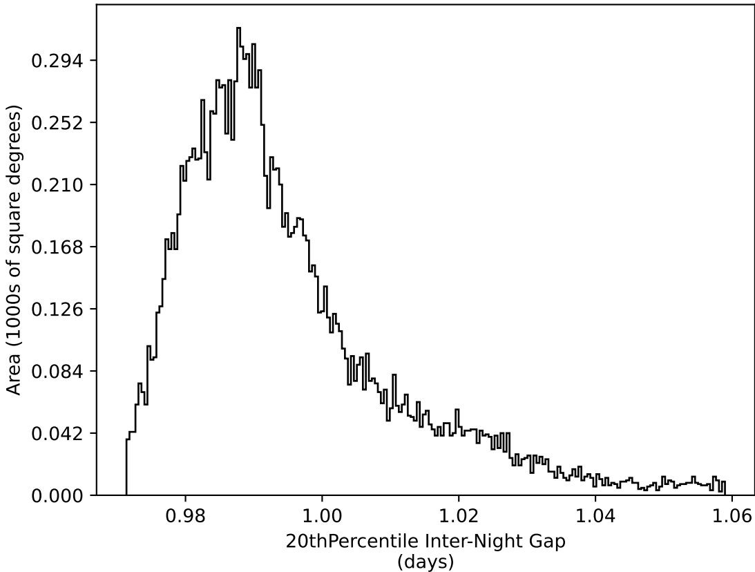
all_long_v3.4_10yrs WFD all bands: 20thPercentile Inter-Night Gap
