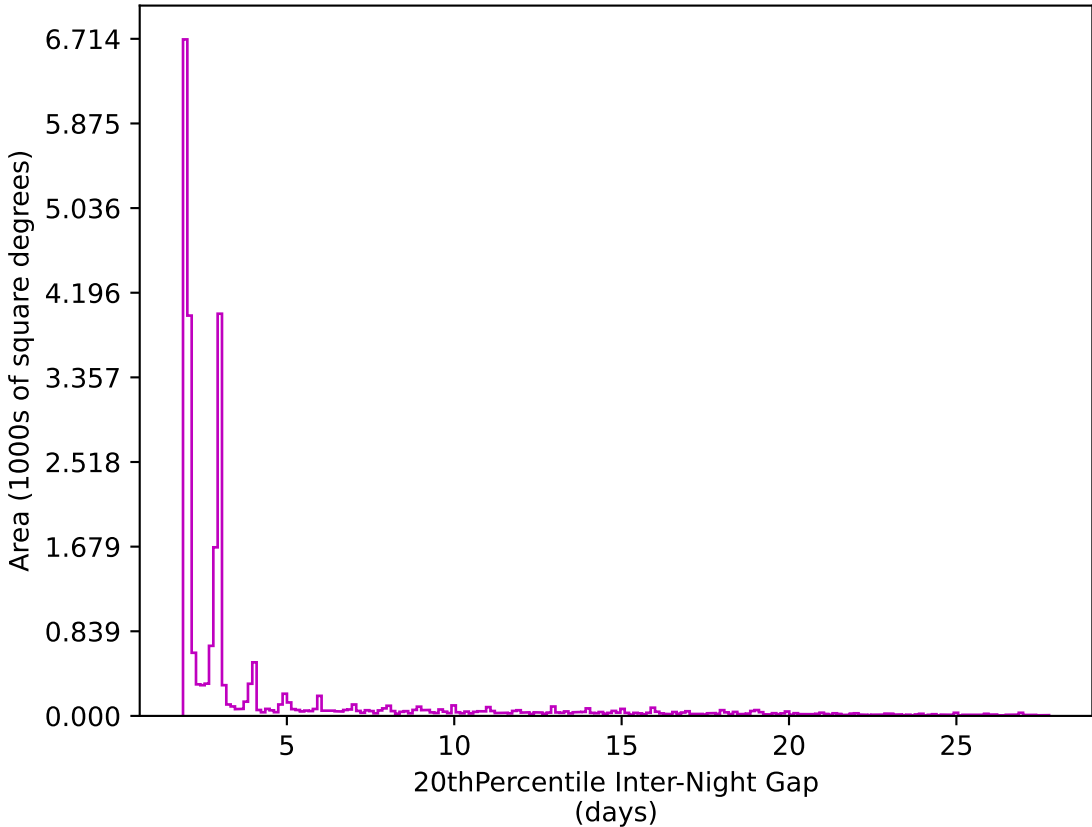
all_long_v3.4_10yrs All sky z band: 20thPercentile Inter-Night Gap
