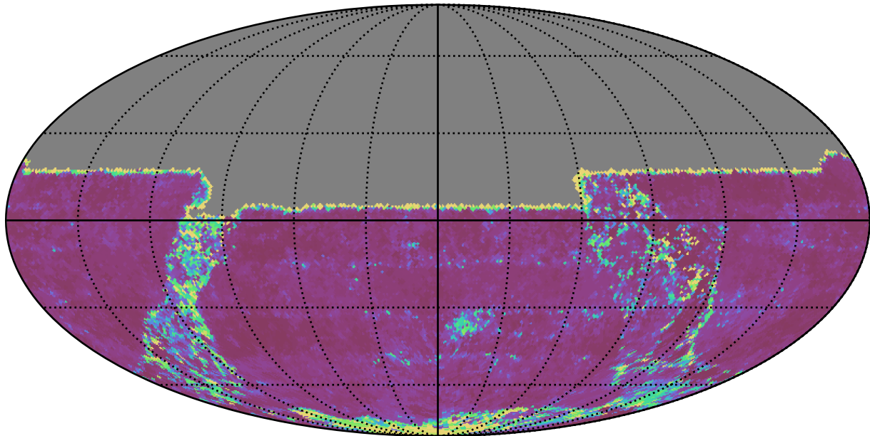
all_long_v3.4_10yrs All sky u band: 20thPercentile Inter-Night Gap
